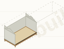
5. Wall framing — the method
