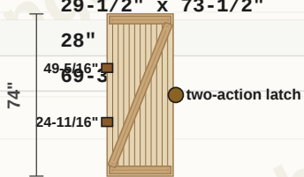
Diagonal runs UP from the hinge side. Hinge heights measured from the bottom of the slab.
