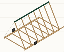
3. Rib assembly — the rafter ...
