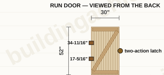
Diagonal runs UP from the hinge side. Hinge heights measured from the bottom of the slab.
