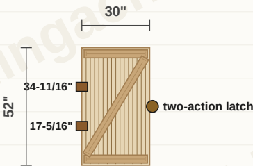
RUN DOOR — VIEWED FROM THE BACK
