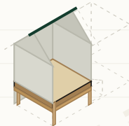
6. Gable ends, rafters and rafters
